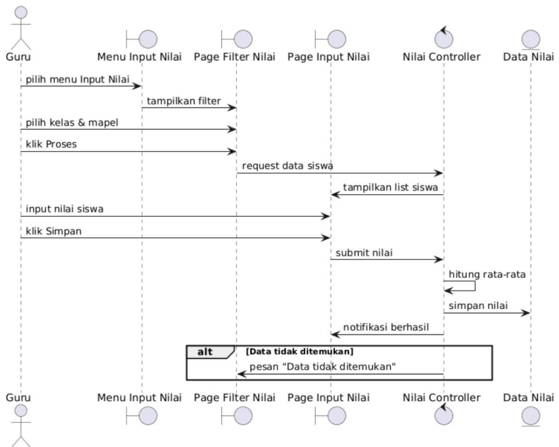
Sequence Diagram - Input Nilai
