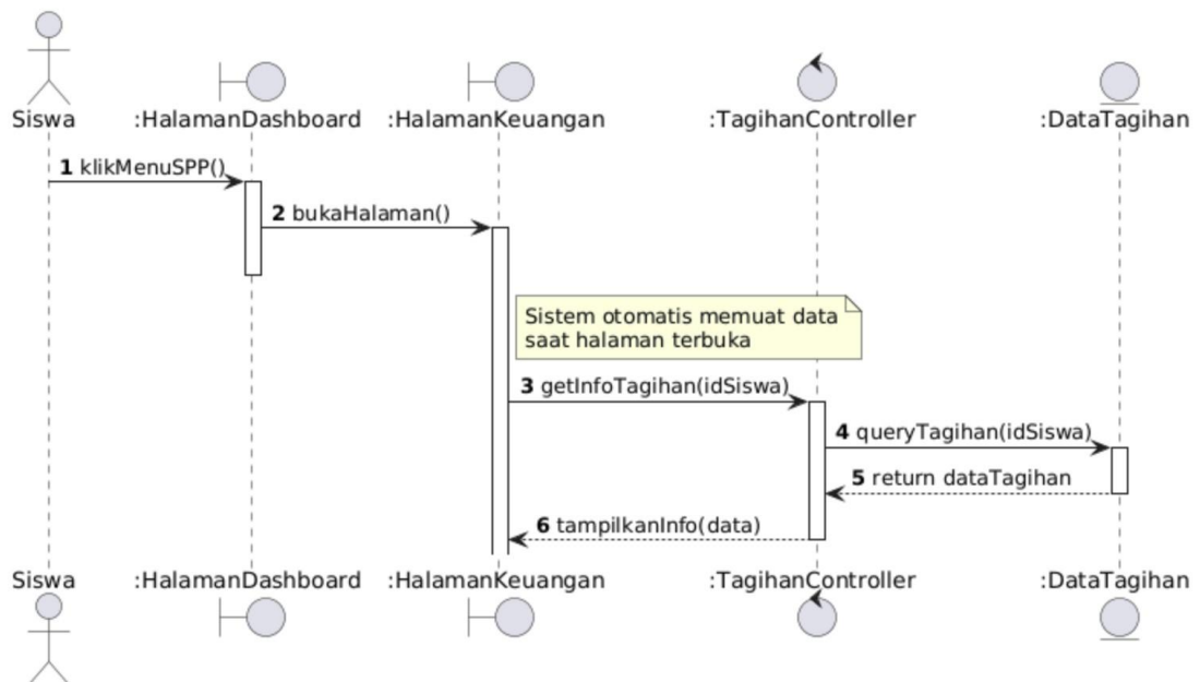
Sequence Diagram - Melihat Tagihan SPP
